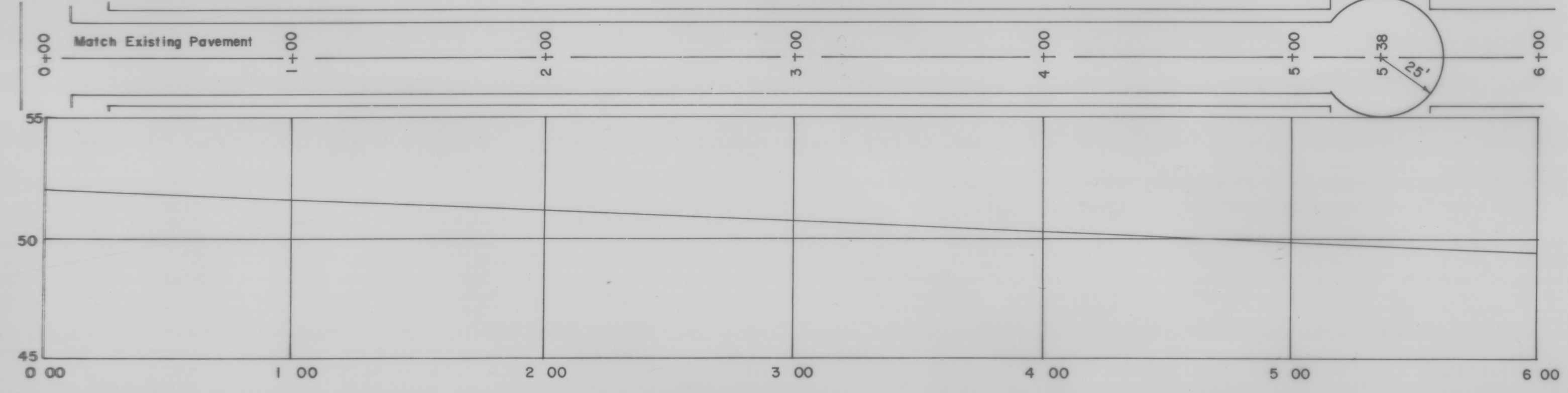
Plan & Profile Pennsylvania Avenue
