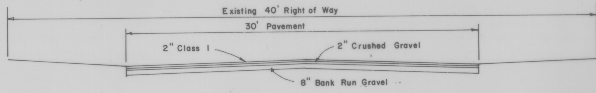
Typical Section Pennsylvania Avenue
