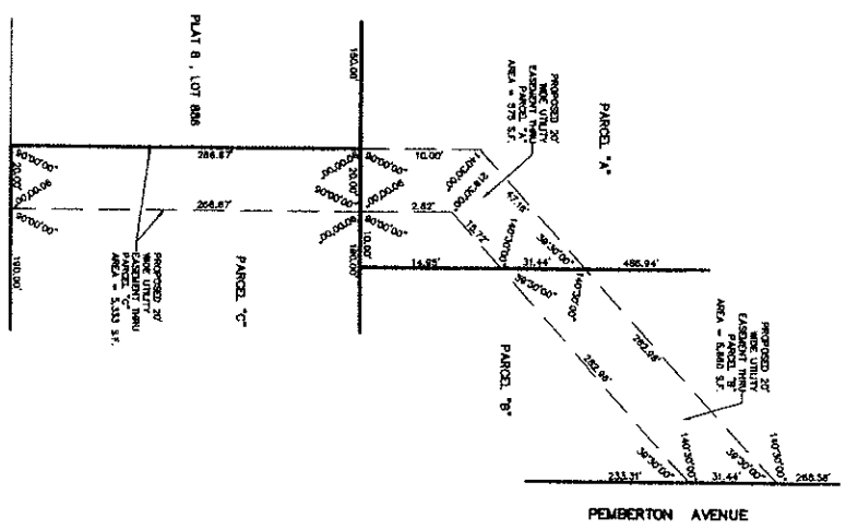
UTILITY EASEMENT DETAIL NOT TO SCALE
