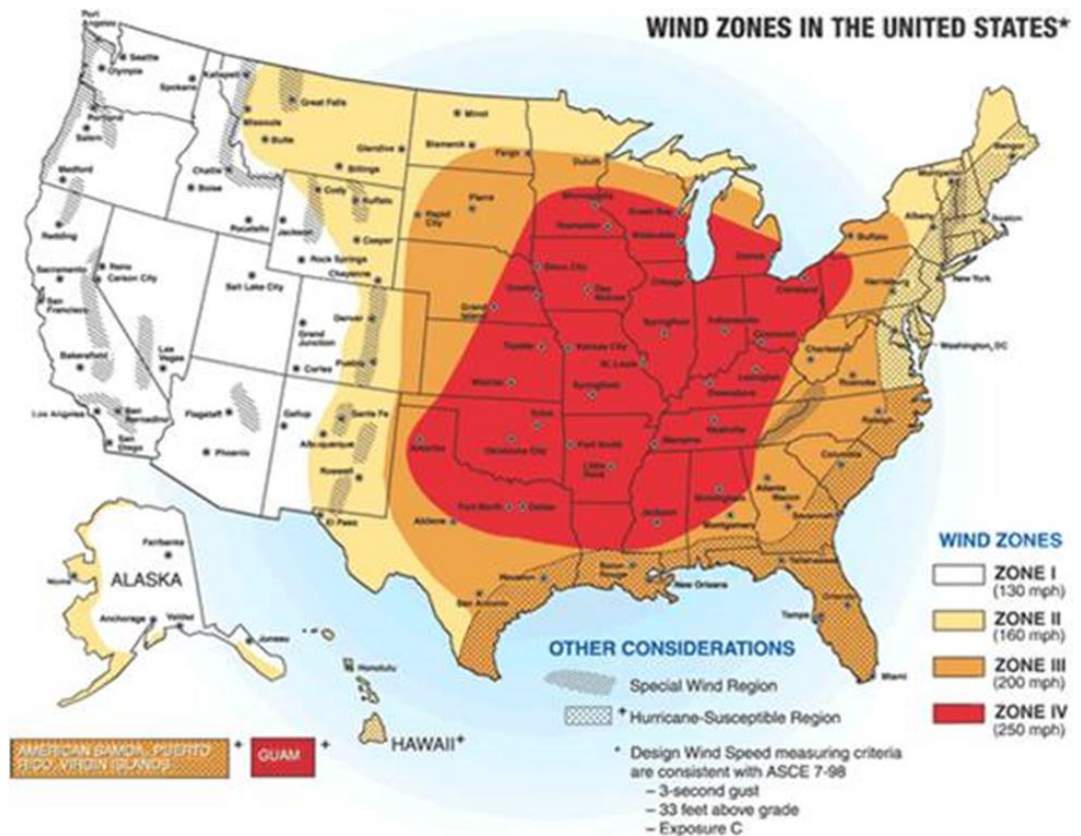
Figure 3-1 Wind Zones in the United States
